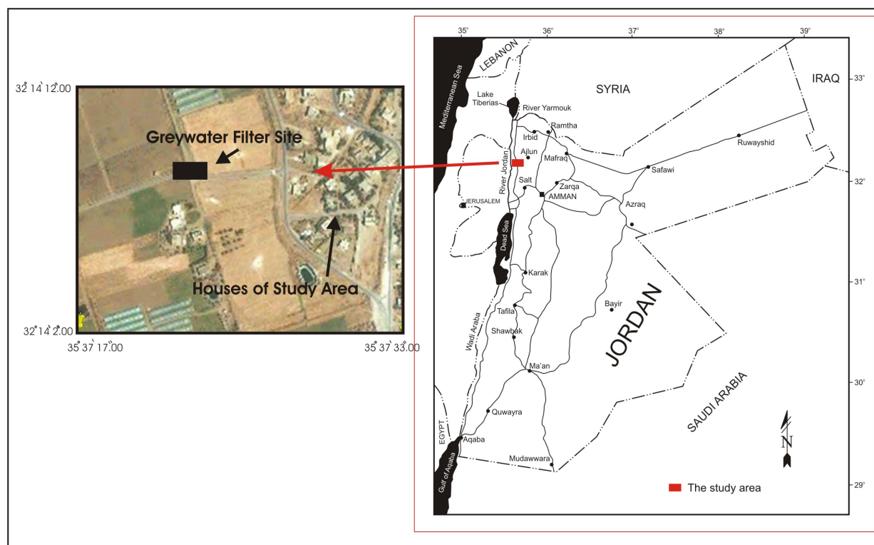
Figure 1. Location map of the studied area, DeirAlla, Jordan (Um-Ayyaash area).
