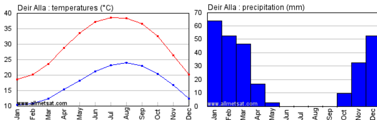
Figure 2. Average annual precipitation and temperature for Deir Alla region [28].
